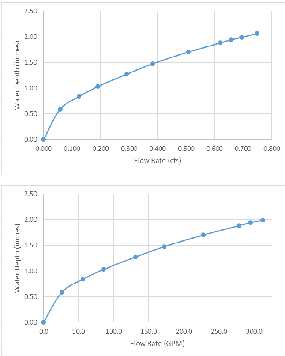
Figure 1, Rating curve
