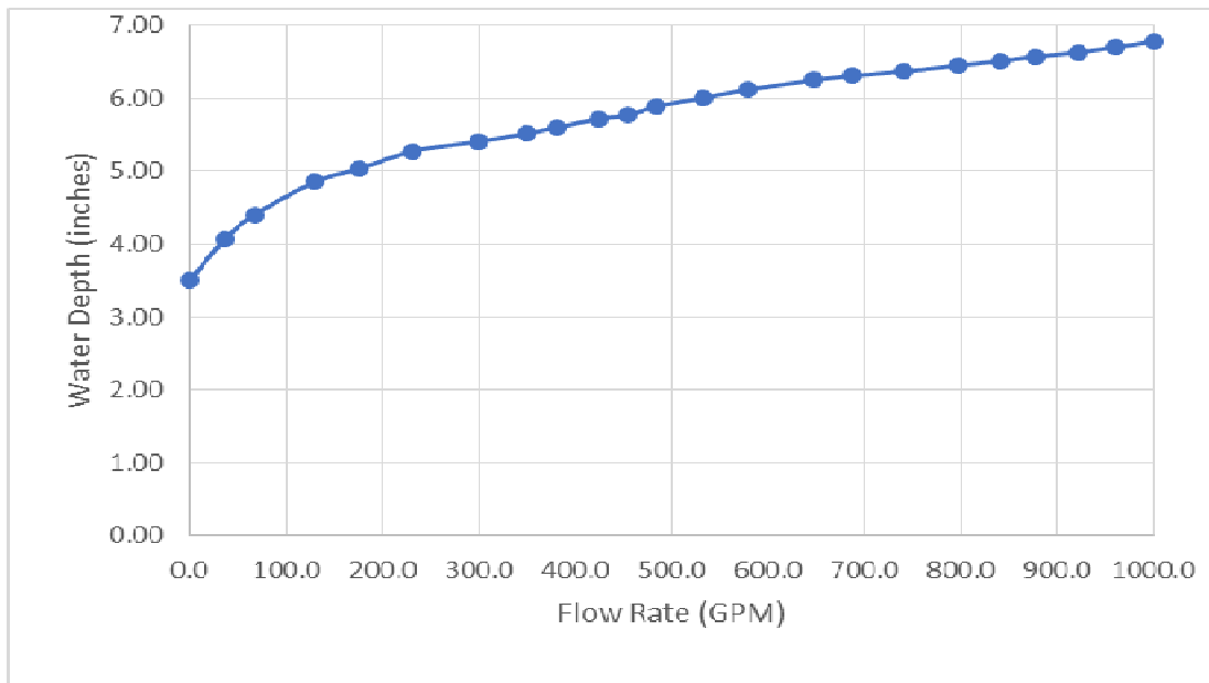
Figure 1, Rating curve
