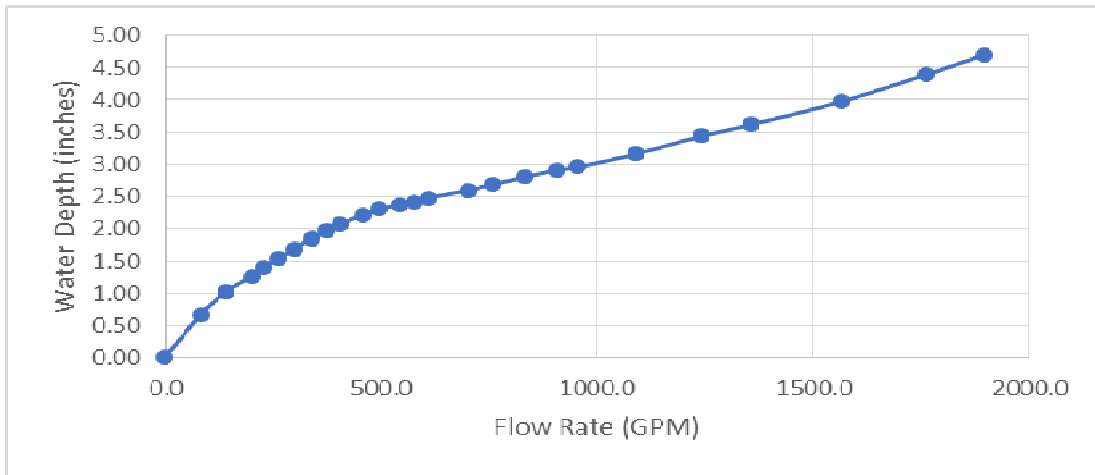
Figure 1, Rating curve
