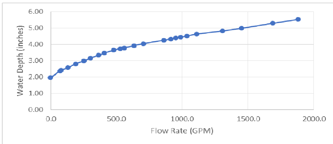
Figure 1, Rating curve
