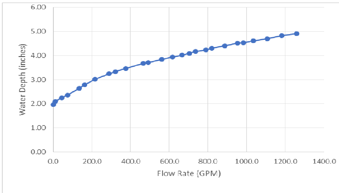
Figure 1, Rating curve
