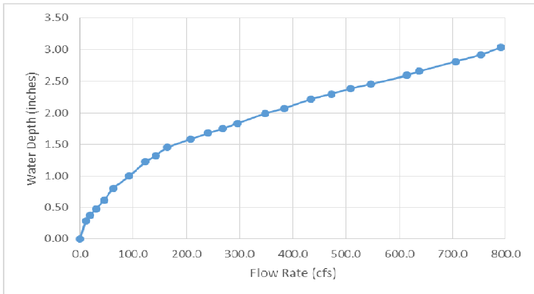
Figure 1, Rating curve
