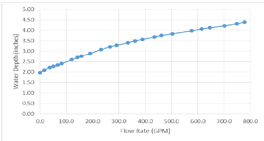
Figure 1, Rating curve
