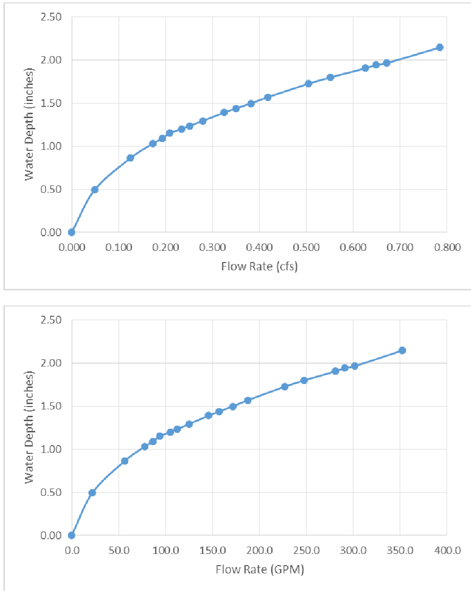
Figure 1, Rating curves
