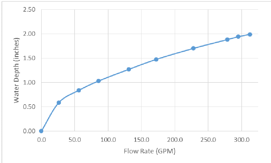
Figure 1, Rating curve
